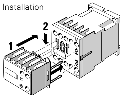
Fig. 3-44: Solid-state time relay block with semiconductor output, installation (frame size S00)
