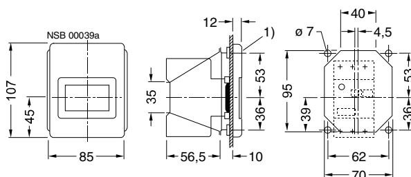
Fig. 2-54: 3RV19 13-4C (frame size S00)
