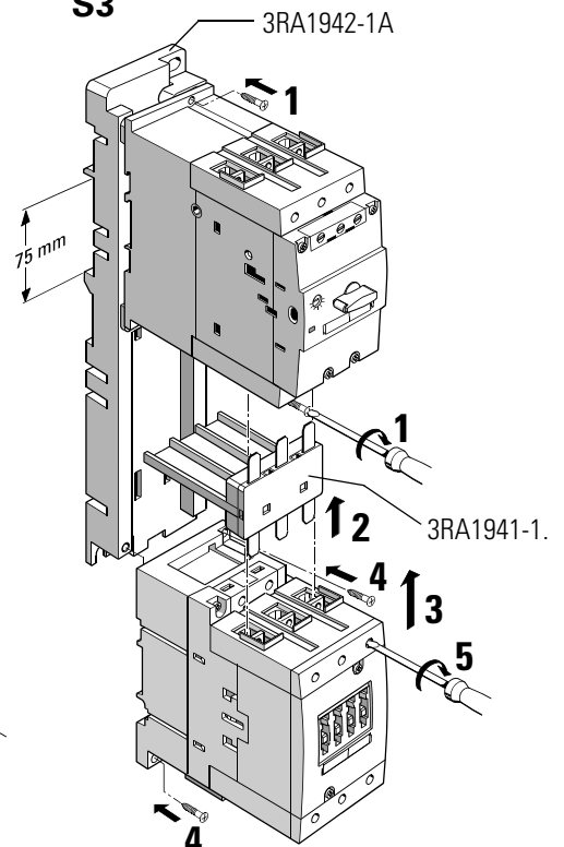
Fig. 5-4: Self-assembly, rail, direct starter (frame sizes S00 to S3)
