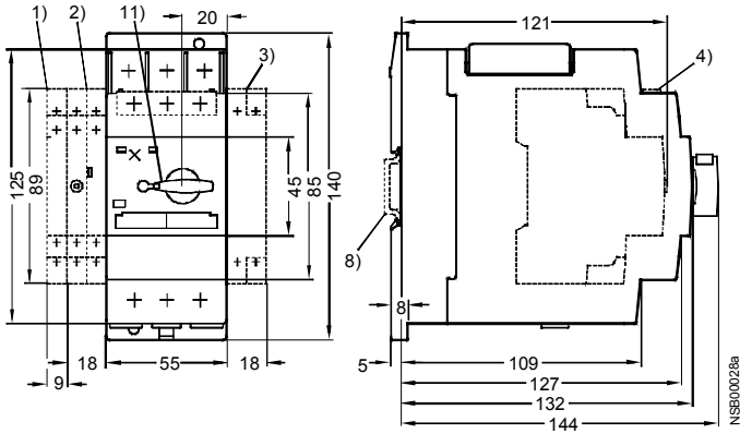
Fig. 2-41: 3RV10 31, 3RV13 31, 3RV14 31 (frame size S2)
