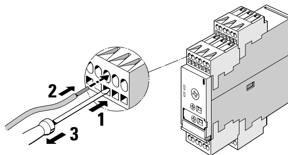
Fig. 7-18: Connection of the springloaded terminal
