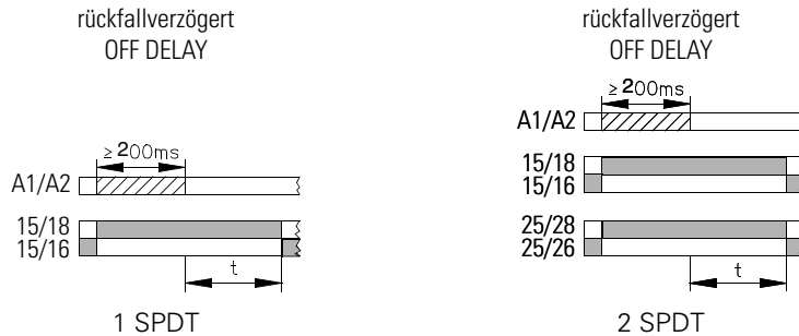
Fig. 7-11: 3RP15 40 Function diagram
