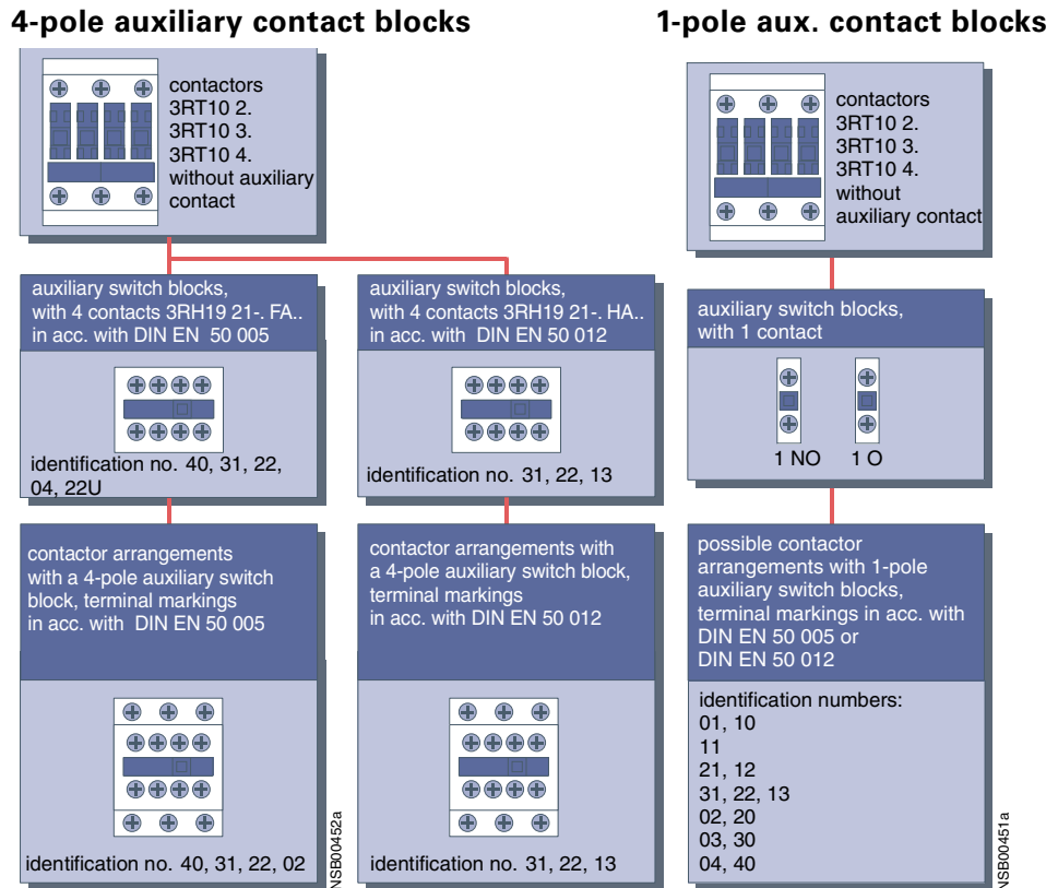
Fig. 3-32: Auxiliary contacts for contactors for the switching of motors (frame sizes S0 to S3)
