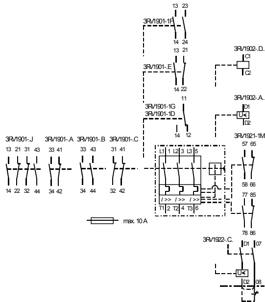
Fig. 2-37: Device circuit diagram (frame sizes S0 to S3, example: circuit breaker (MSP) for motor protection 3RV10)
