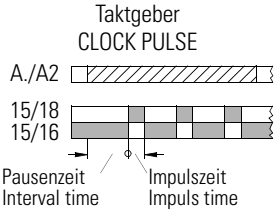
Fig. 7-12: 3RP15 55 function diagram
