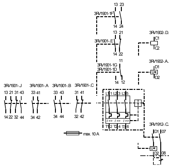
Fig. 2-36: Device circuit diagram (frame size S00, example: circuit breaker (MSP) for motor protection 3RV10)
