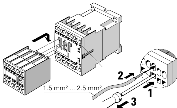
Fig. 3-69: Cage Clamp terminals
