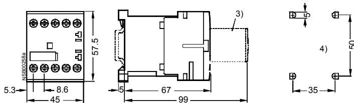
Fig. 3-87: 3RT10 1. with surge suppressor Different dimensions for coupling contactors with Cage Clamp-connection: height 60 mm
