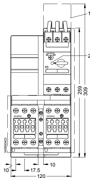
Fig. 5-27: 3RA1 reversing operation (frame size S0)
