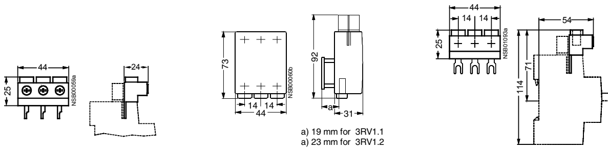
Fig. 2-73: 3RV19 15-5A Connection from above (for frame size S00)
