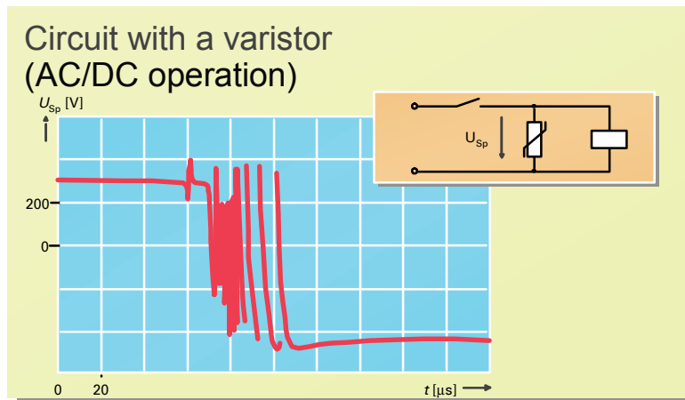
Fig. 3-53: Circuit with a varistor (AC/DC operation)
