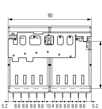
3RT1916-4KA2 attached to S00 device with front mount auxiliary contact block
