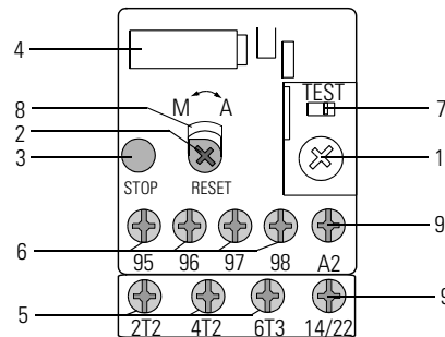
Fig. 4-1: Front view 3RU11 3RB10 is the same as 3RU11 with exception of the integrated sealable cover.
