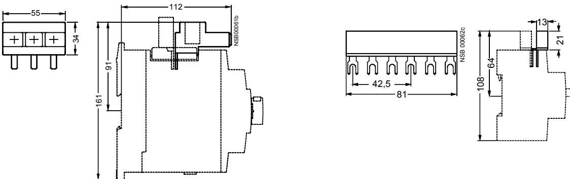
Fig. 2-76: 3RV19 35-5A Connection from above (for frame size S2)
