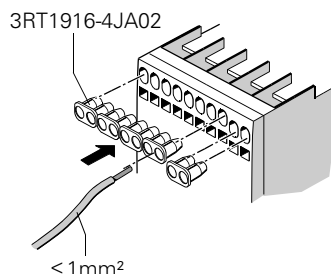
Fig. 1-9: Conductor cross-sections \leq 1 \text{ mm}^2
