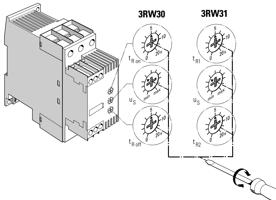
Fig. 8-16: Settings, 3RW3
