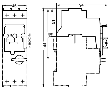
Fig. 2-46: 3RV19 28-1A (for frame size S0)
