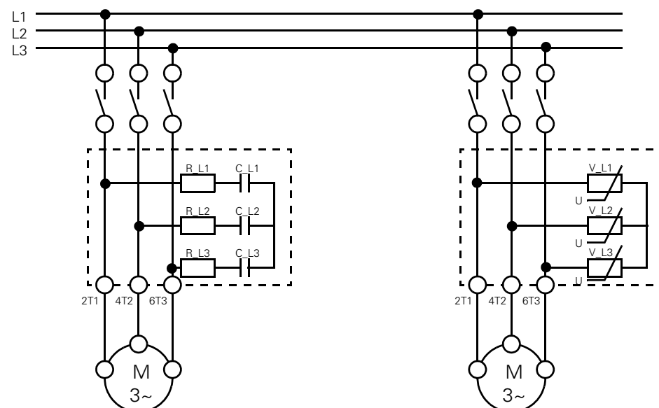
Fig. 3-58: Circuit diagrams
