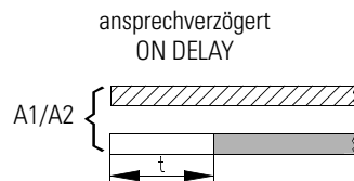
Fig. 7-9: 3RP15 27 Function diagram
