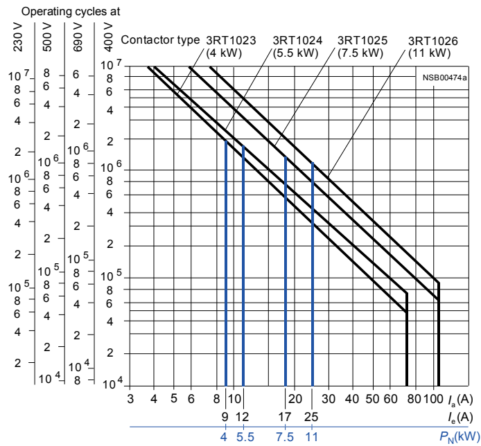
Fig. 3-4: Characteristic curve of the electrical service life of the main contacts (frame size S0)
