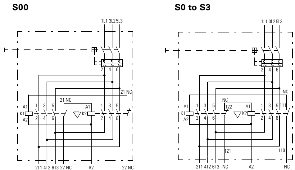
Fig. 5-15: Circuit diagrams, reversing starters (frame sizes S00 to S3)
