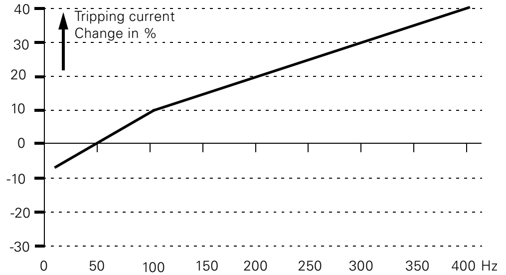
Fig. 2-7: Frequency sensitivity of the short-circuit releases
