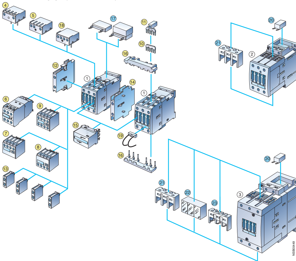
Fig. 3-27: Accessories for contactors of frame sizes S0 to S3
