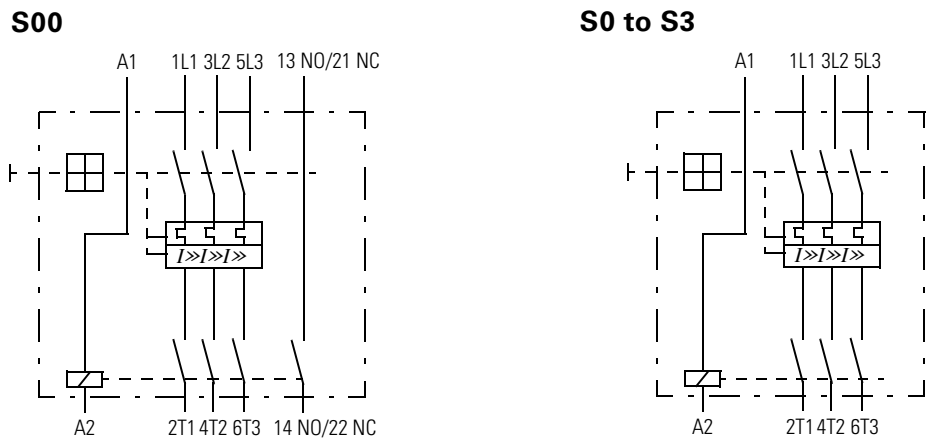
Fig. 5-14: Circuit diagrams, direct starters (frame sizes S00 to S3)
