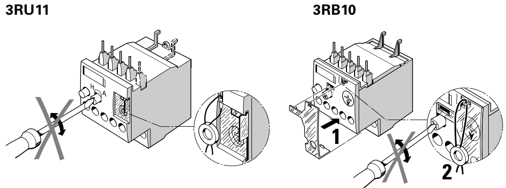
Fig. 4-3: Sealing the current setting dial (frame size S00)
